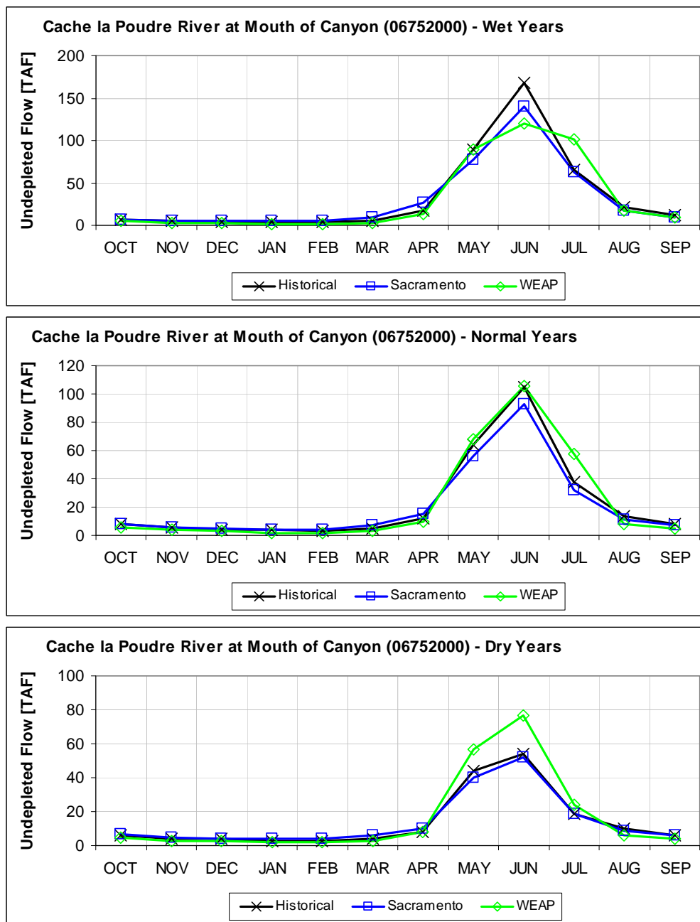
Figure 2.31 Calibration Comparison for the Cache la Poudre at Mouth of Canyon (Monthly Average)
